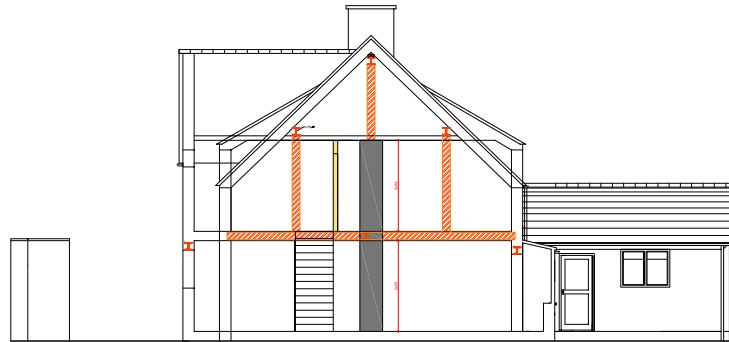
Proposed West Elevation: Section A-A
