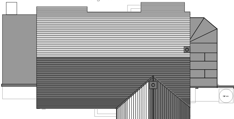
Existing Roof Plan
